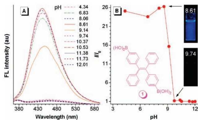
Figure 1. (A) FL spectra of 1 (10 \mu M) in Britton–Robinson buffers containing 2 vol % DMSO at different pH values. (B) Change in the FL intensity ( I ) of 1 at 440 nm with pH; I_0 is the intensity at pH 12.01. Inset: photographs of the mixtures of 1 in the aqueous buffers at pH 8.6 and 9.7 taken under the illumination of a hand-held UV lamp ( \lambda_{\text{ex}} = 365 nm).
