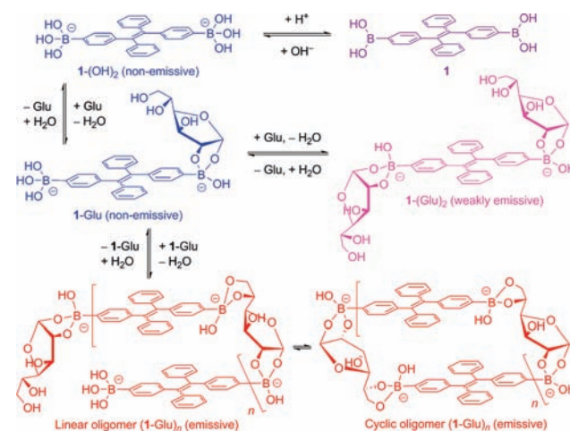
Figure 1. (A) FL spectra of 1 (10 \mu M) in Britton–Robinson buffers containing 2 vol % DMSO at different pH values. (B) Change in the FL intensity ( I ) of 1 at 440 nm with pH; I_0 is the intensity at pH 12.01. Inset: photographs of the mixtures of 1 in the aqueous buffers at pH 8.6 and 9.7 taken under the illumination of a hand-held UV lamp ( \lambda_{\text{ex}} = 365 nm).
