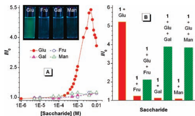
Figure 2. (A) Variation in the FL intensity ( I ) of 1 (50 \mu M) at 485 nm as a function of the concentration of saccharide in a carbonate buffer containing 2 vol % DMSO (pH 10.5). I_0 is the intensity in the absence of a saccharide. Inset: photographs of solutions of 1 in carbonate buffers containing 5 mM saccharide taken under UV illumination. (B) FL responses of 1 (50 \mu M) to saccharides (4 mM; red solid bars) or to Glu in the presence of another saccharide interferent (0.1 mM; green shaded bars).
