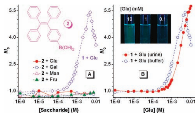
Figure 3. Variations in the FL intensities ( I ) of mixtures of (A) 2 ( 10 \mu\text{M} ) with various concentrations of saccharides in the carbonate buffer containing 10 vol % DMSO and (B) 1 ( 50 \mu\text{M} ) with Glu in artificial urine. I_0 is the intensity in the absence of saccharide. In each panel, FL data for 1 ( 50 \mu\text{M} ) in the carbonate buffer containing Glu is shown for comparison. The inset in panel B shows photographs of mixtures of 1 ( 50 \mu\text{M} ) in the artificial urines containing different amounts of Glu taken under UV illumination.
